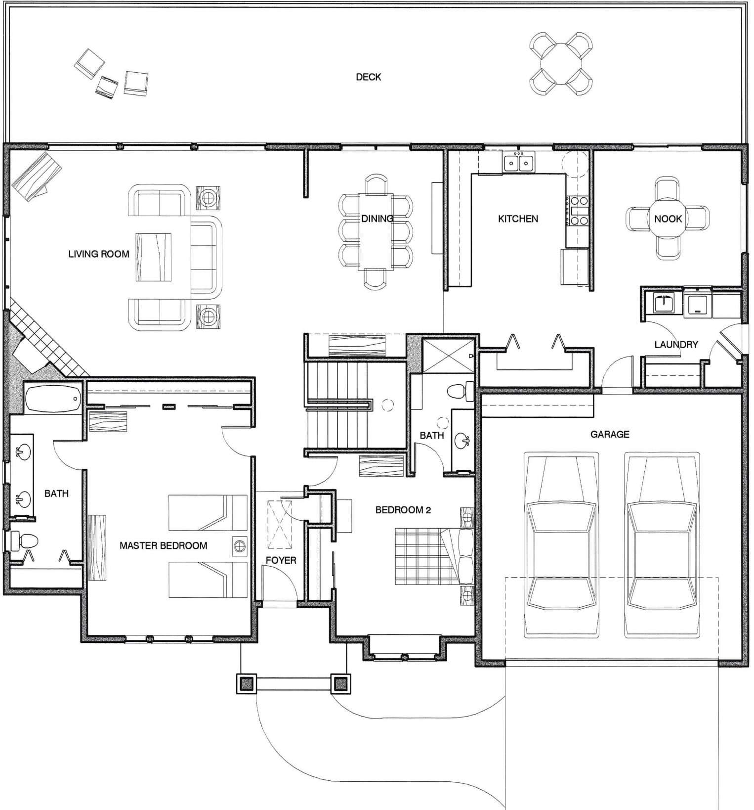
Main Floor Plan 2,118 S.F.
